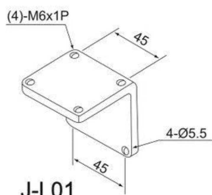
MOUNTING ANGLE PLATE
