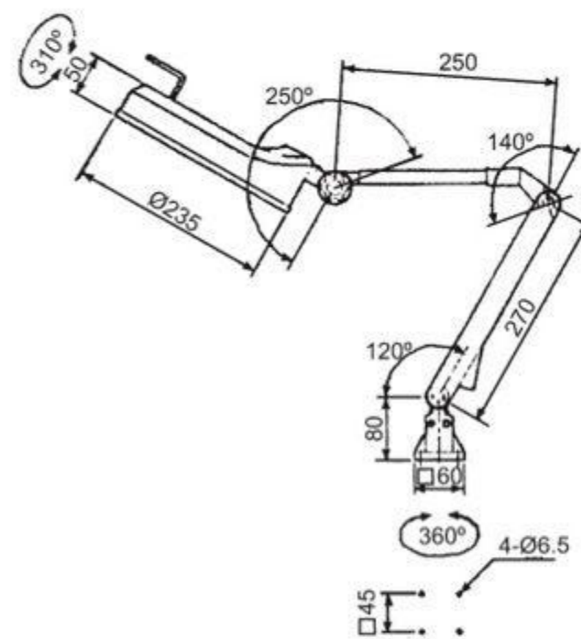
VHL-30MEB MEDIUM ARM
