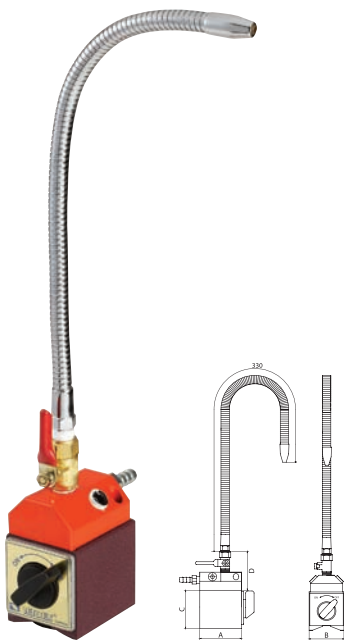
ORDER NO. VMH-63 (1 HOSE) MAGNETIC BASE WITH STEEL NOZZLE
