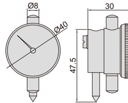
dial indicator
