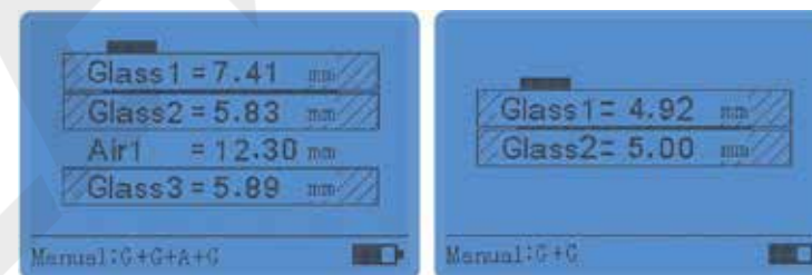
Laminated glass with one layer air
