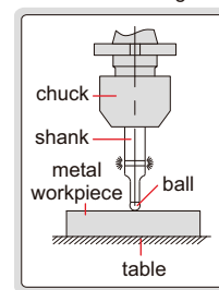
Z axial setting
