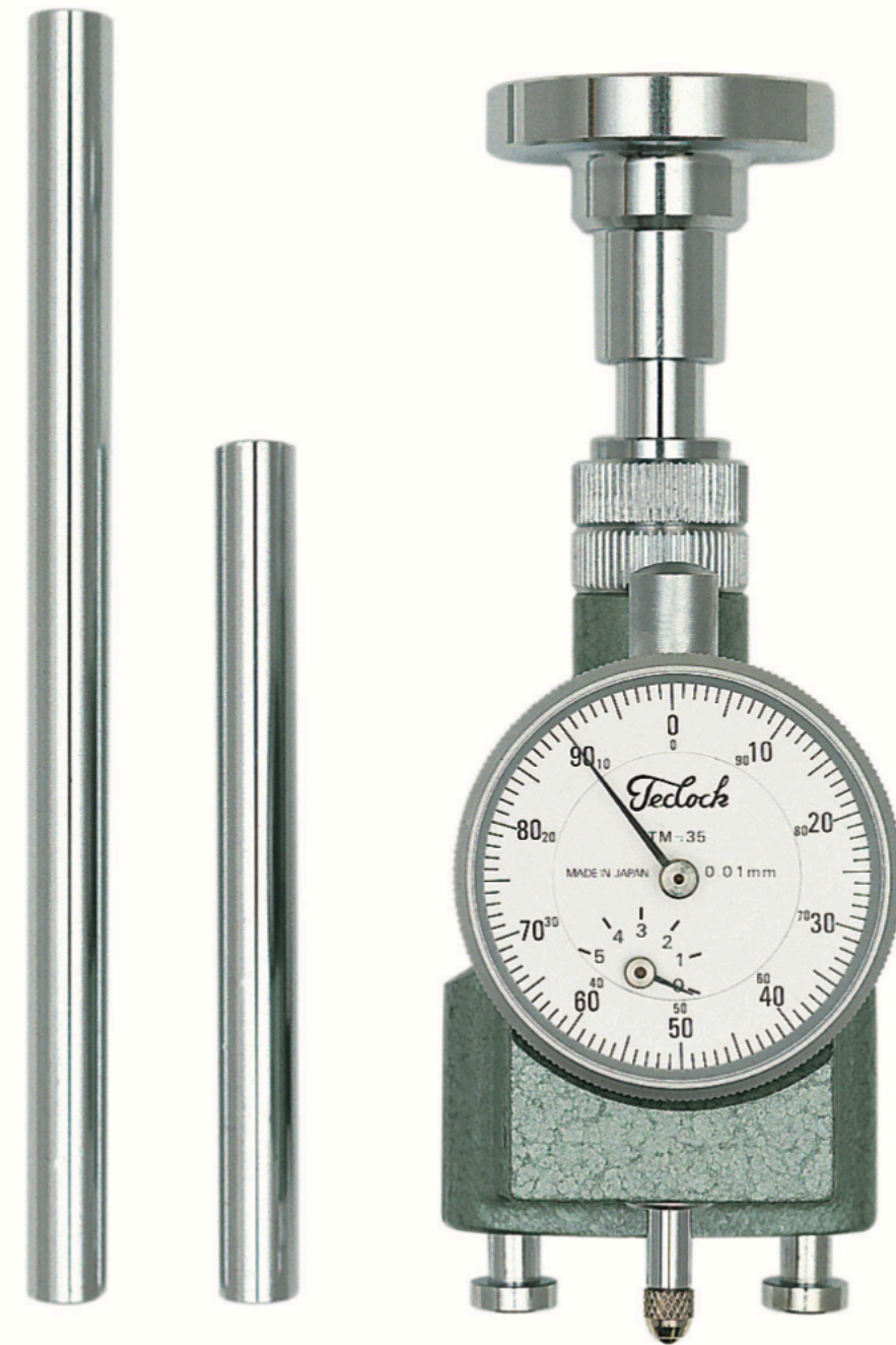
CSDG-A Graduation 0.01mm Measuring Range 110~230mm
