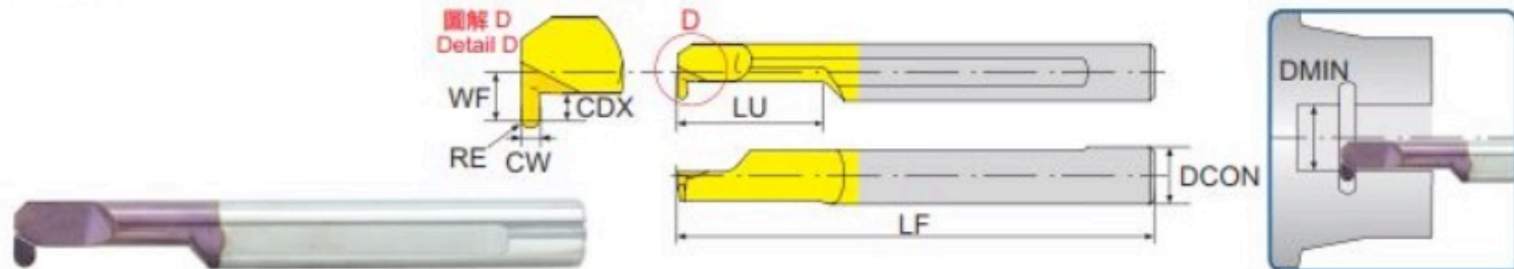
微小徑圓鼻開槽鎢鋼內徑車刀 Tiny Full Radius Grooving Carbide Boring Bar
