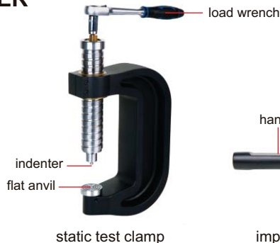
static test clamp
