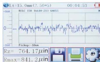
roughness profile
