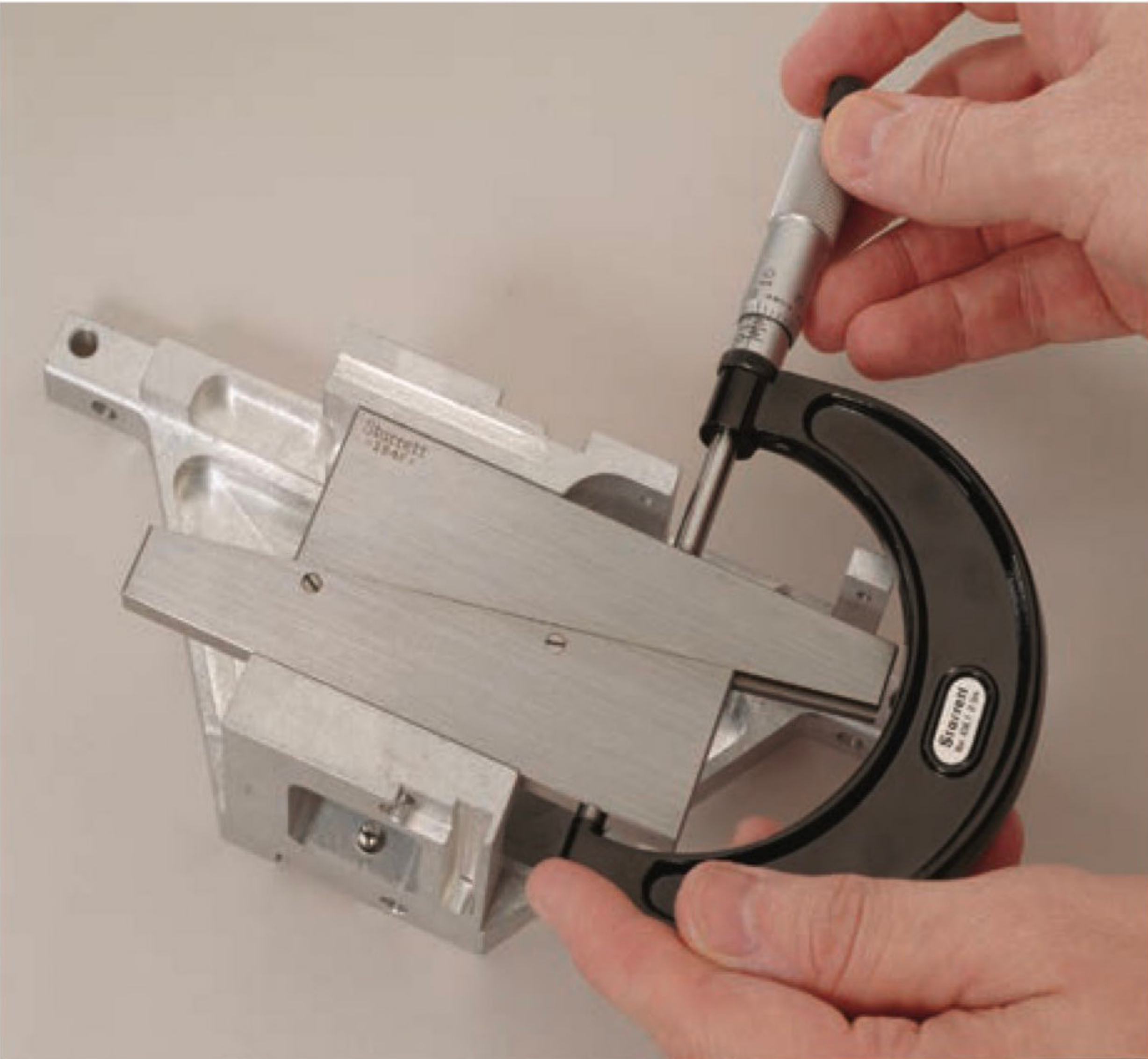
Checking inside measurement of slot with parallel and outside micrometer
