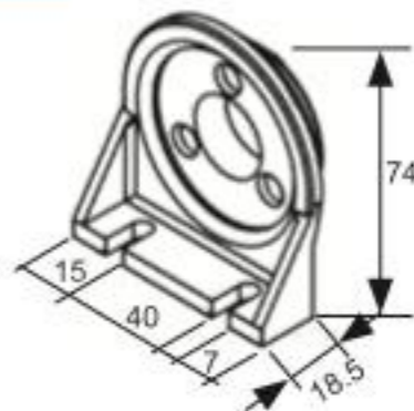
BRACKET
