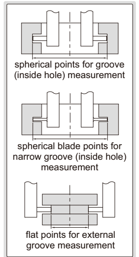
measure internal and external grooves
