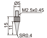
pointed tip
