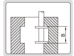
measure width of groove
