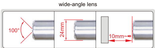
angle of view (θ) diameter (ØD) focus distance (F)
